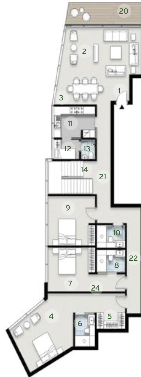
LOWER FLOOR PLAN
